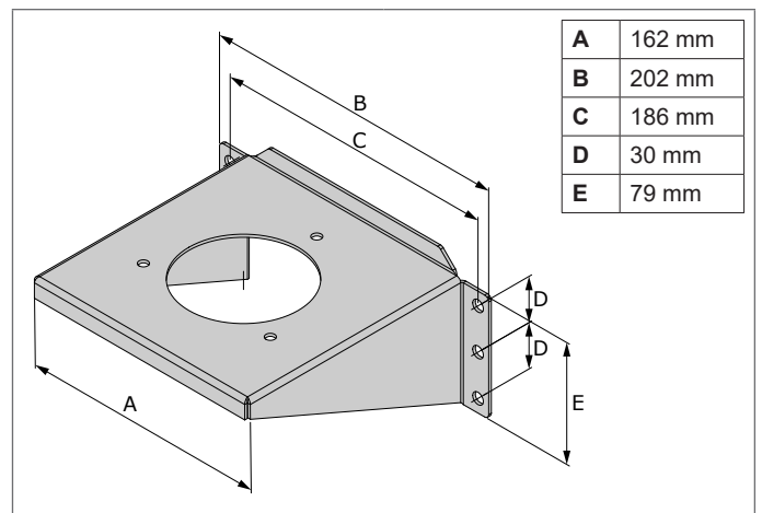
Fig. 4.1 Mounting bracket
