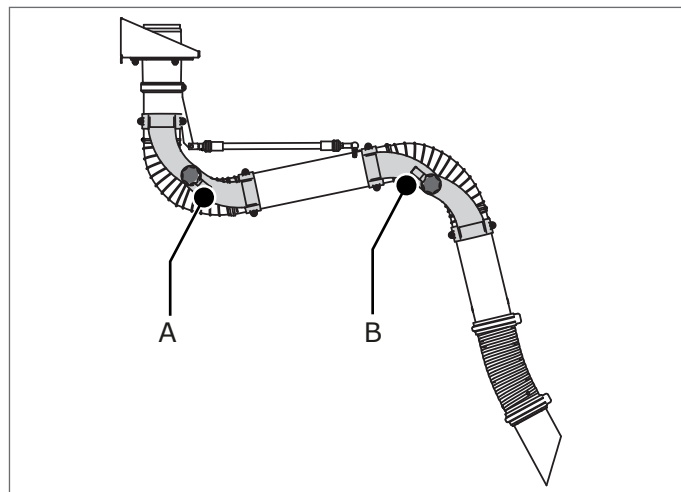
Fig. 6.1 Adjustment points
