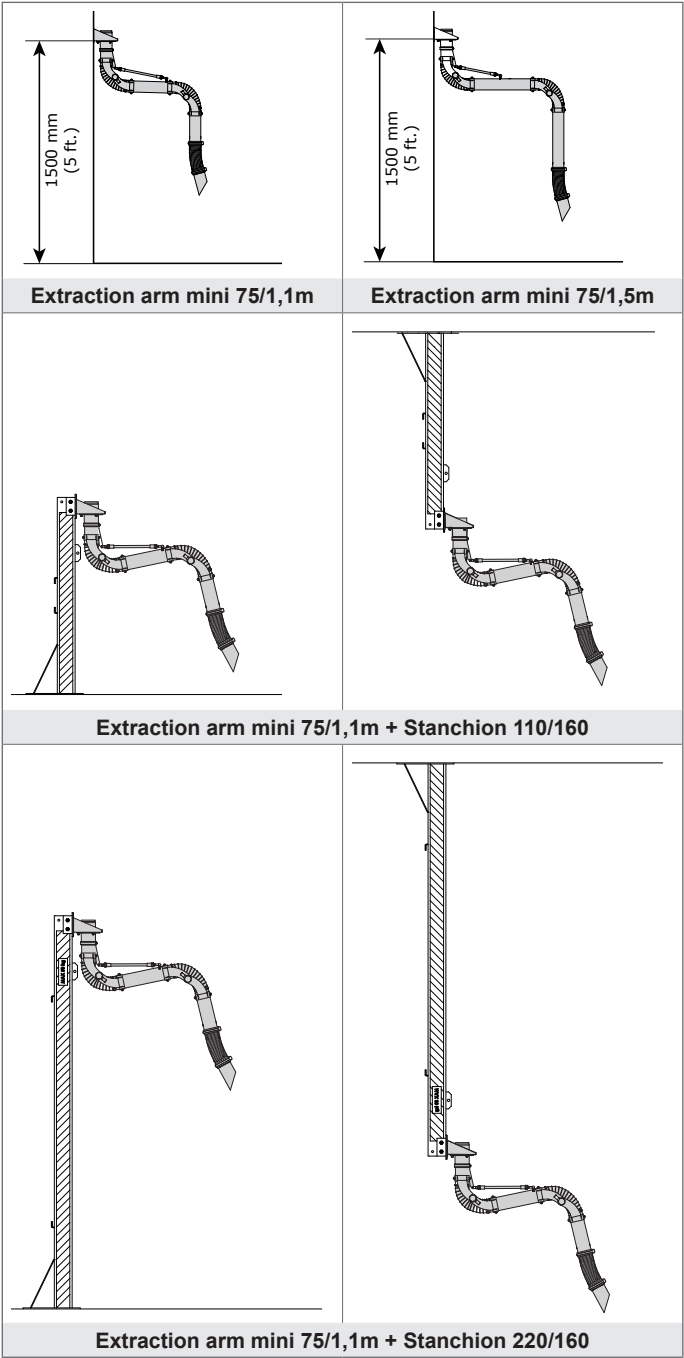
Fig. III Mounting examples
