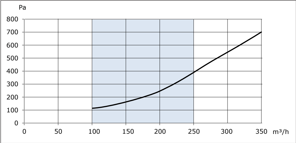
Fig. II Pressure drop
