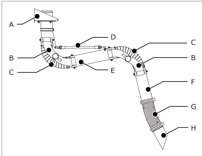
Fig. 2.1 Main components and elements
