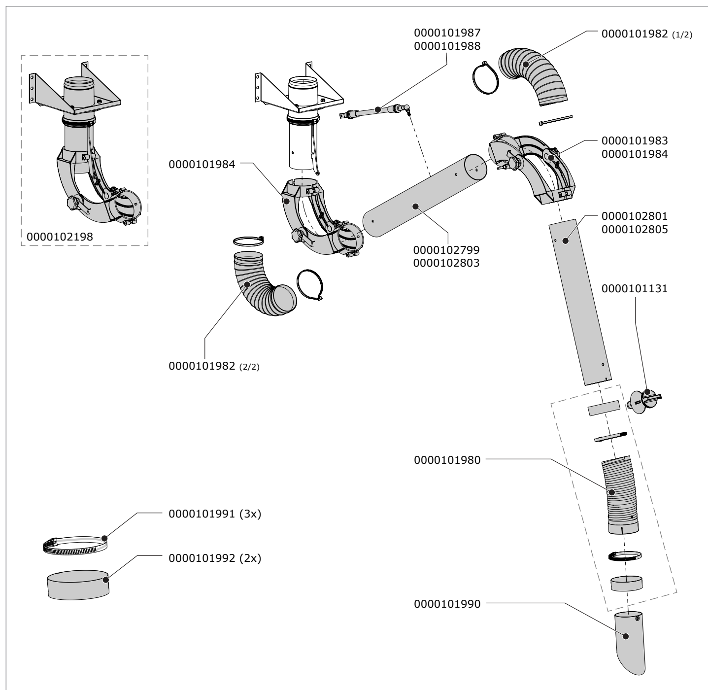
Fig. IV Exploded view | Spare parts
