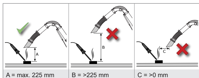
Fig. 5.1 A = Correct position of the nozzle (example: soldering)
