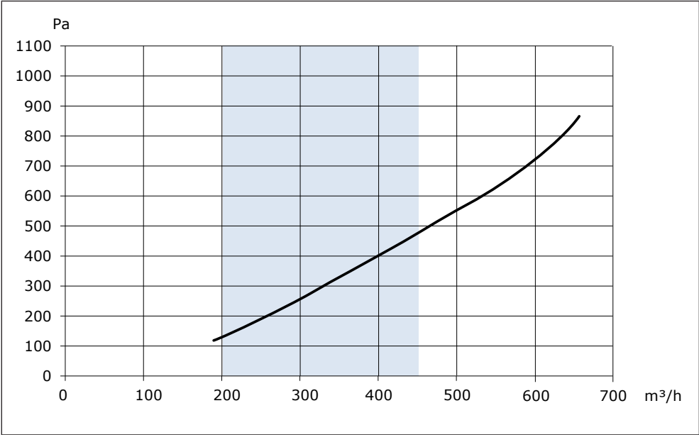
Fig. II Pressure drop
