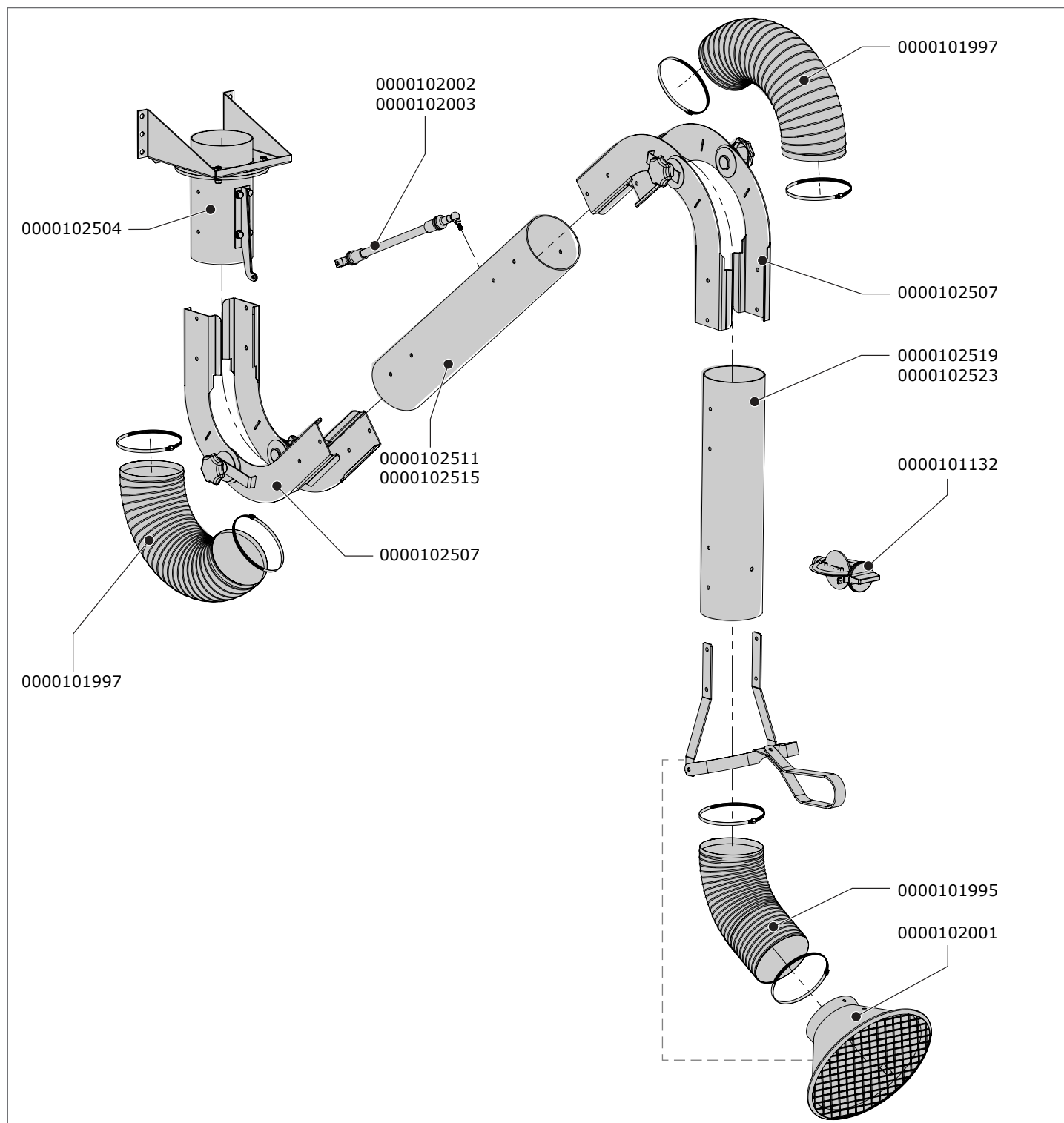
Fig. IV Exploded view | Spare parts
