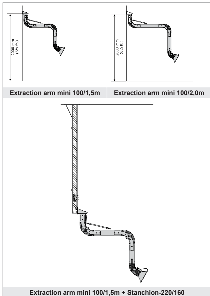
Fig. III Mounting examples
