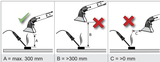
Fig. 5.1 A = Correct position of the hood (example: soldering)
